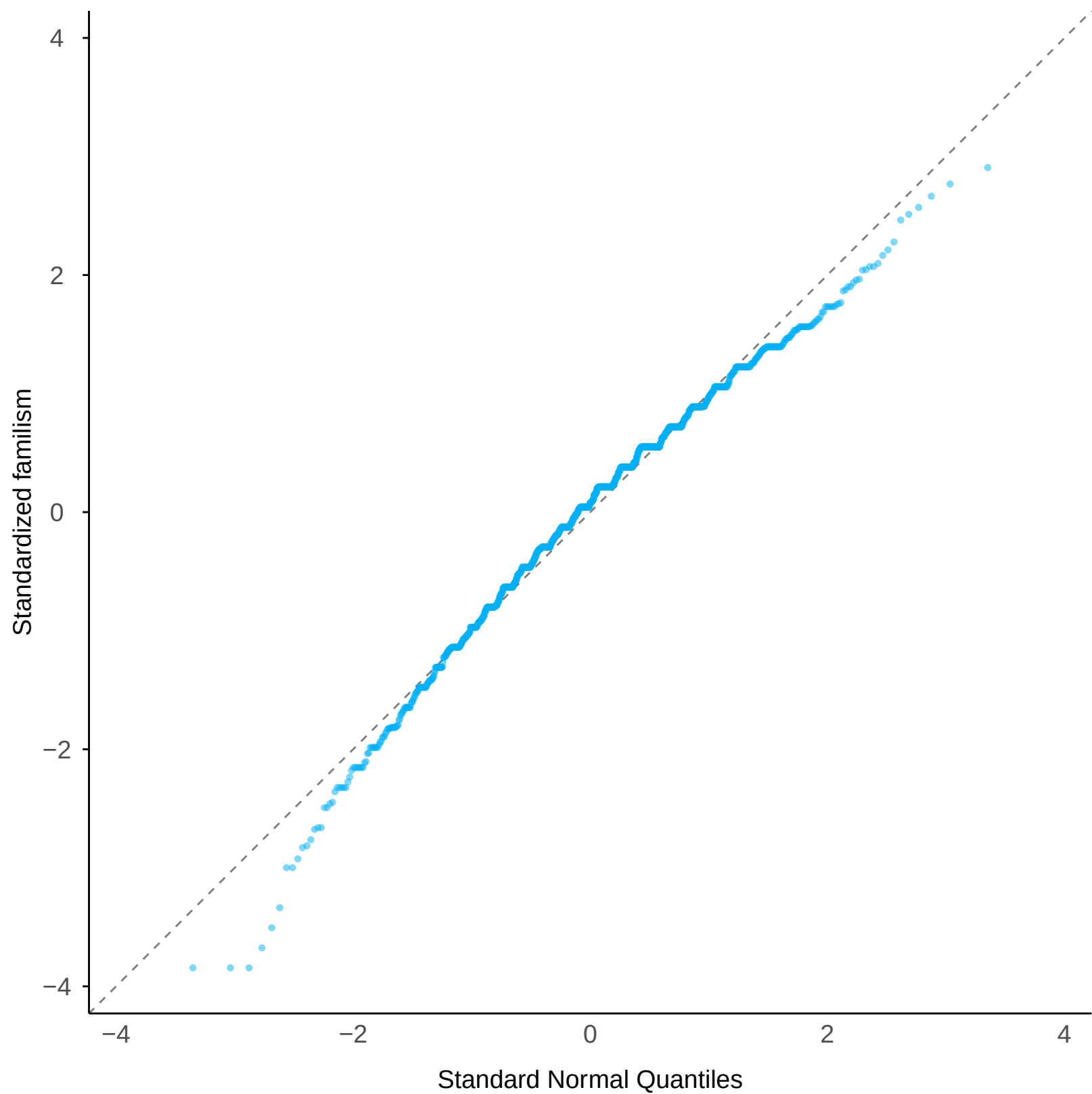
Normal Q-Q: familism
