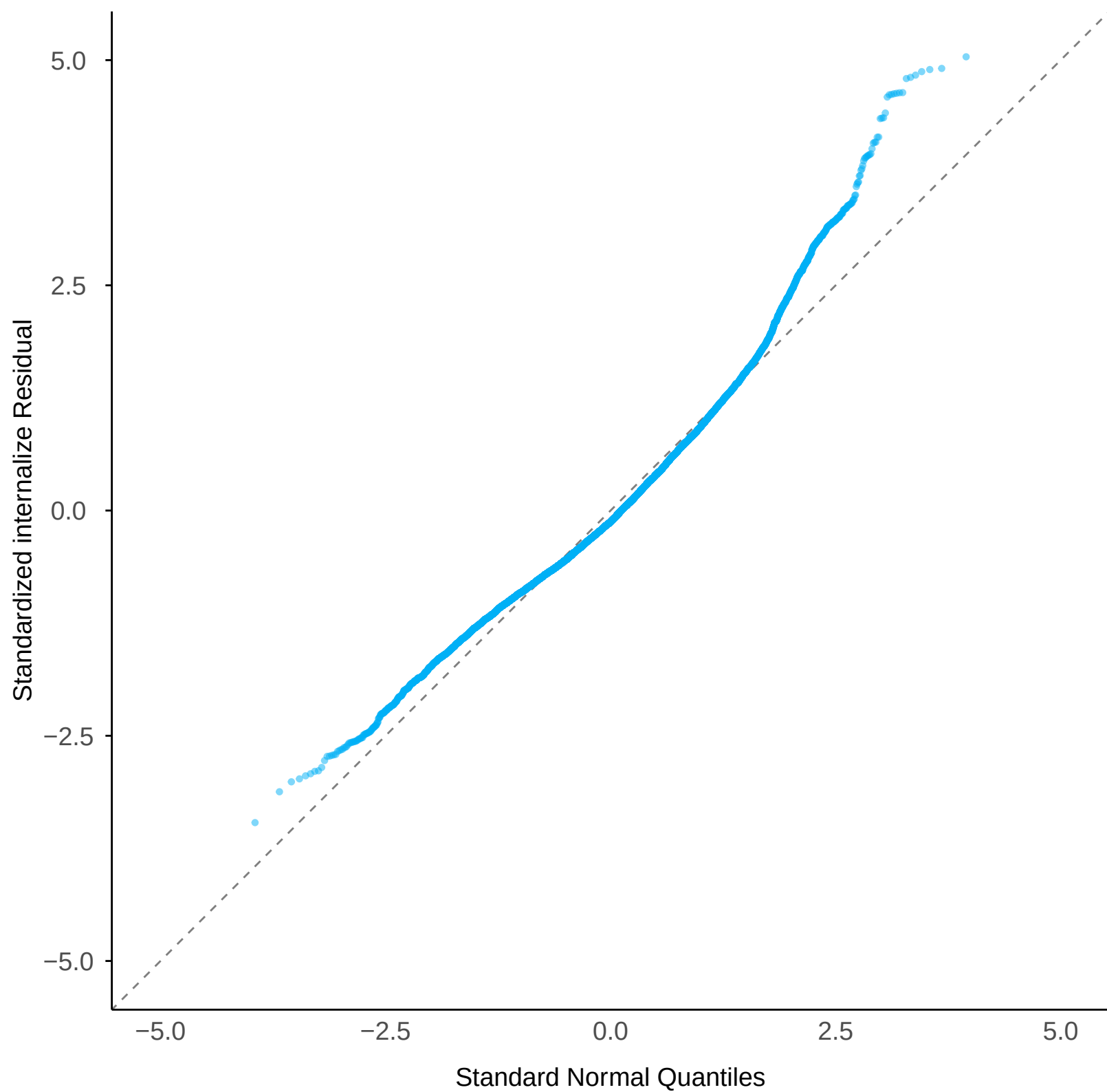
Normal Q-Q: internalize Residual
