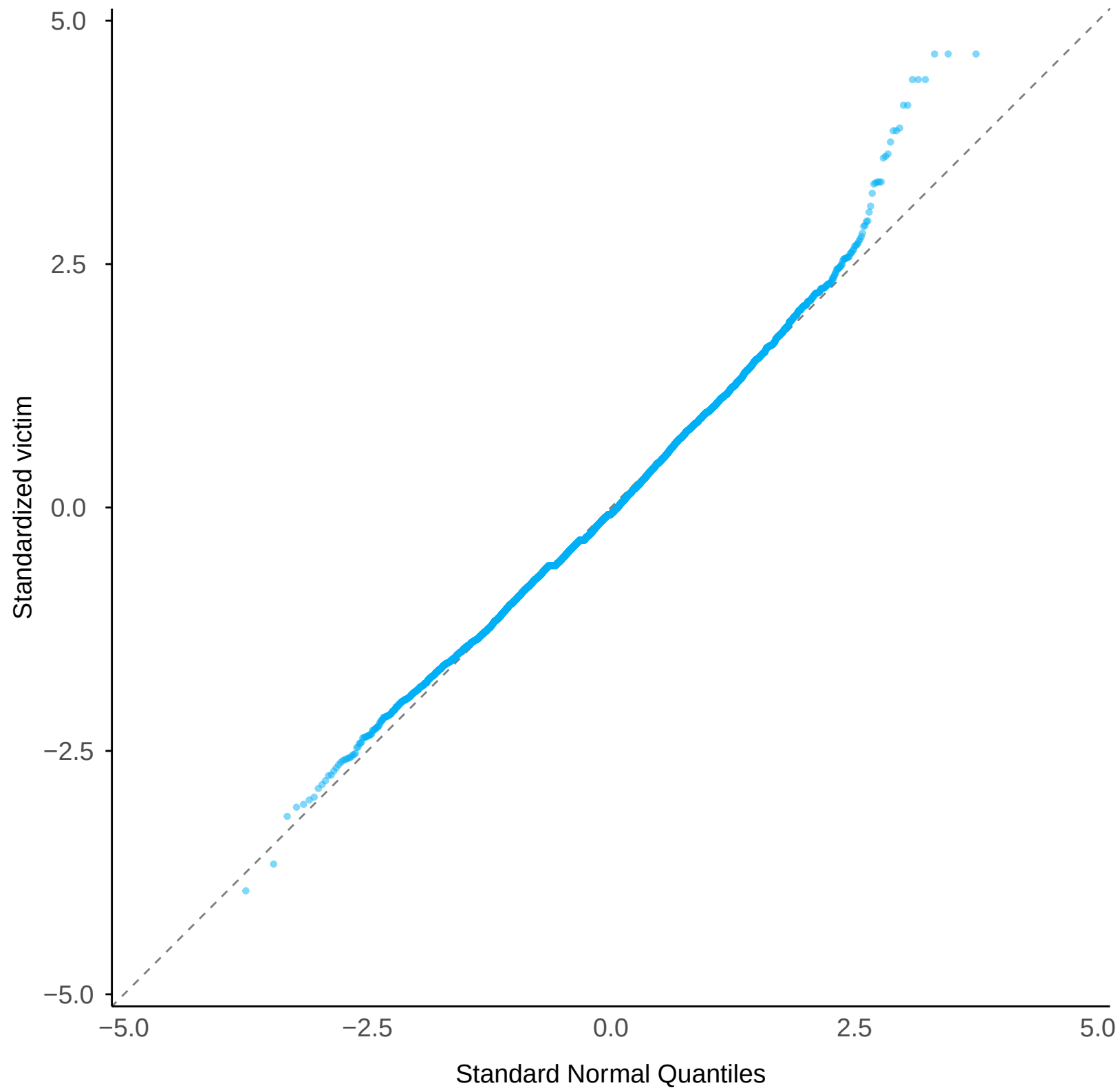
Normal Q-Q: victim
