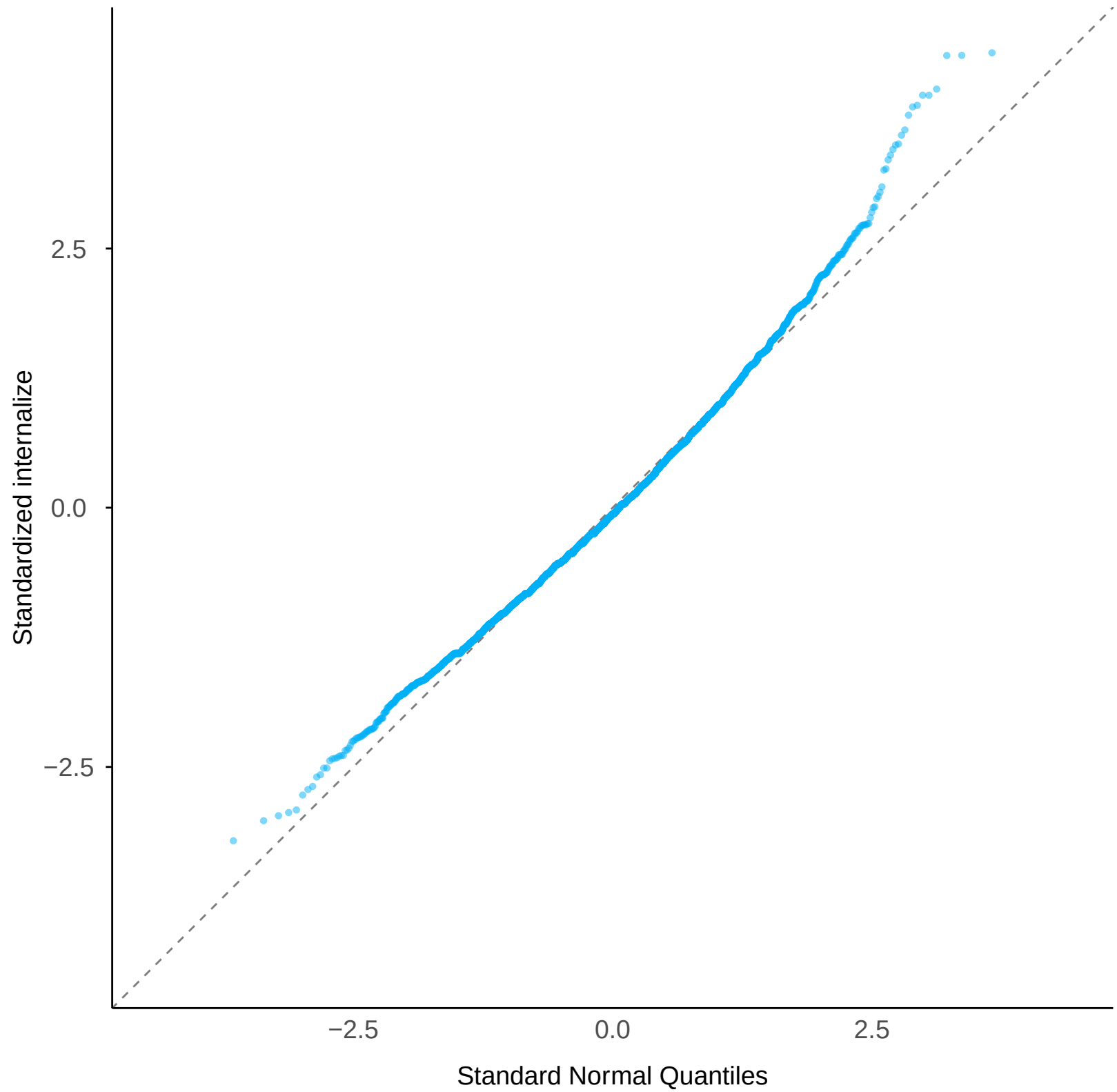
Normal Q-Q: internalize
