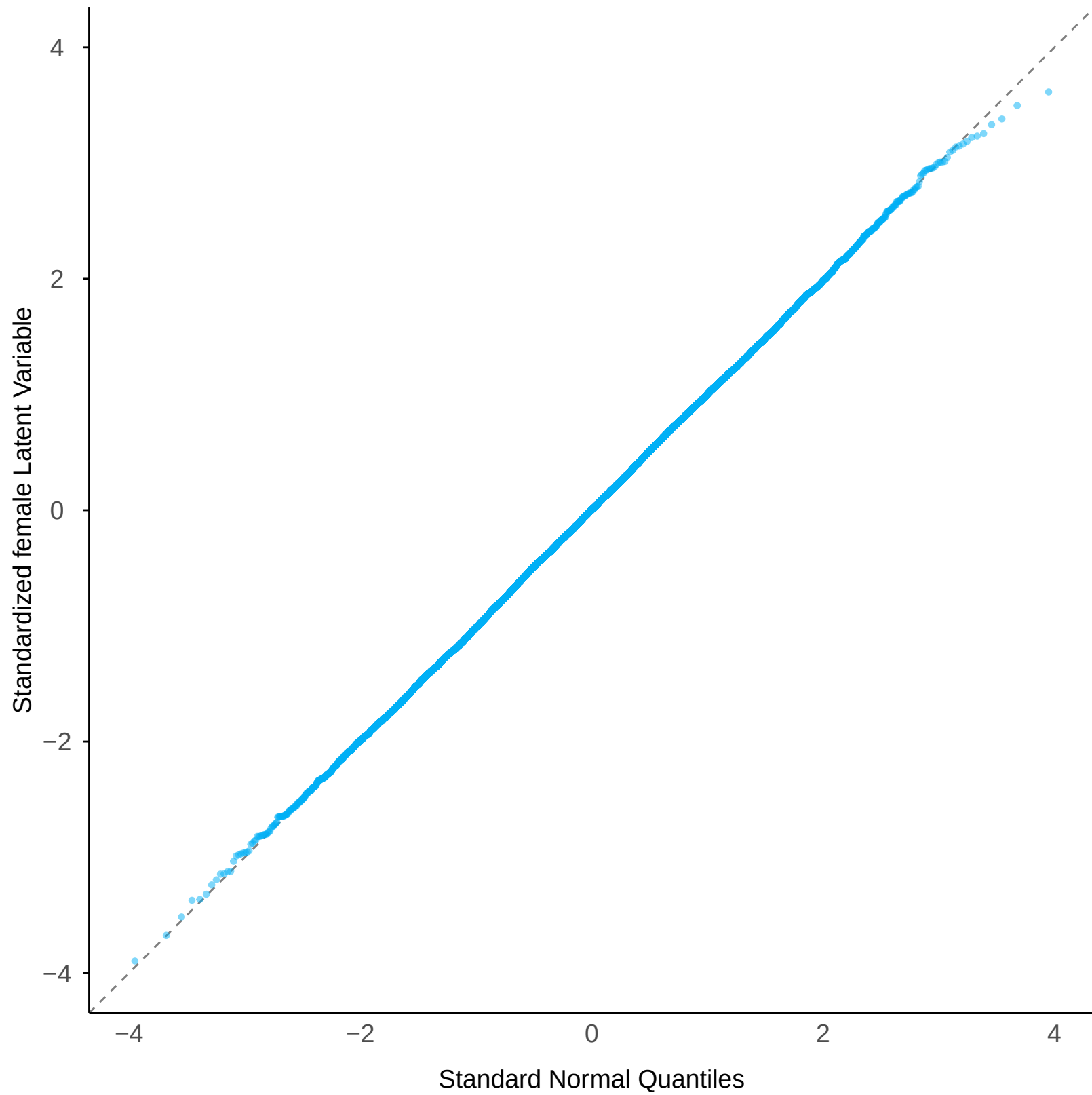
Normal Q-Q: female Latent Variable
