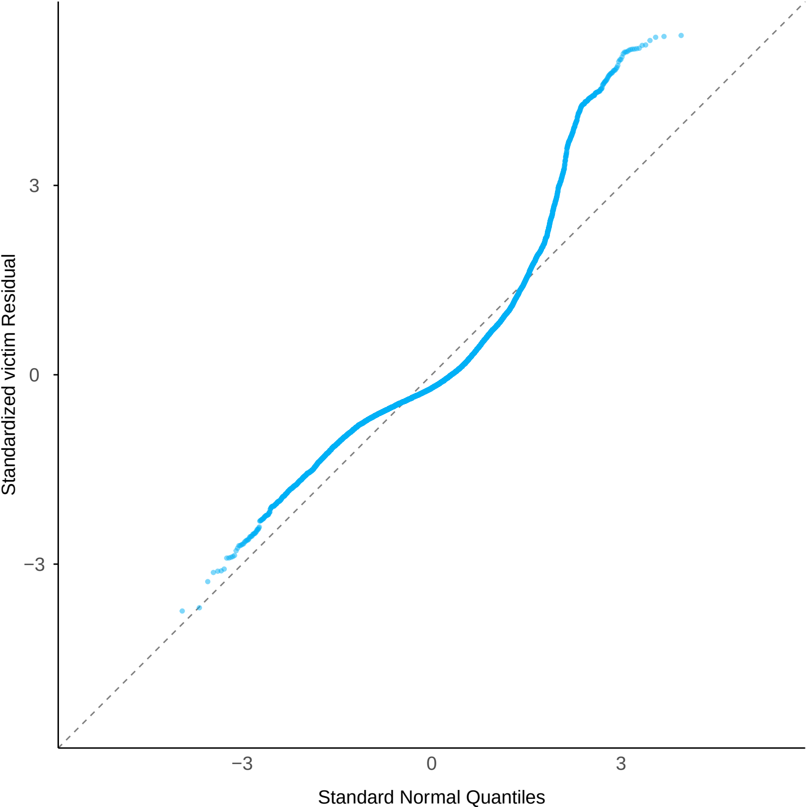
Normal Q-Q: victim Residual
