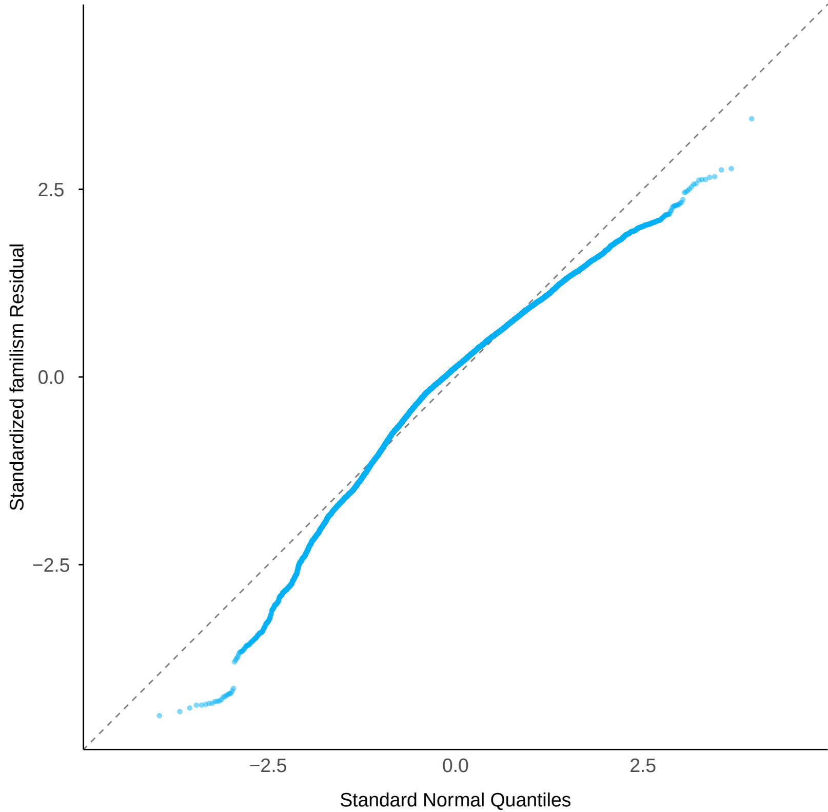
Normal Q-Q: familism Residual
